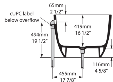
Section BB Shown with K17 Waste Kit
